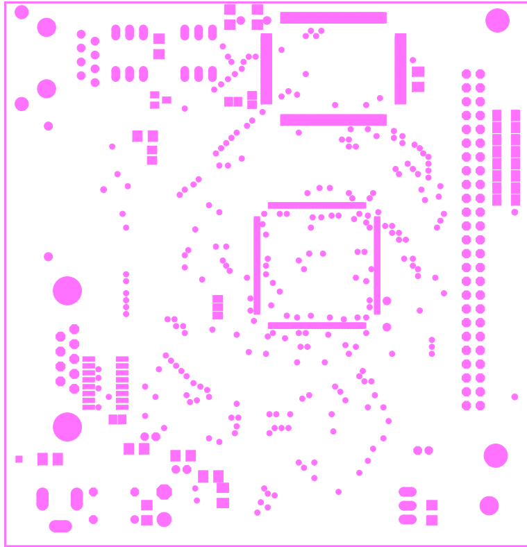
BOTTOM SOLDERMASK
