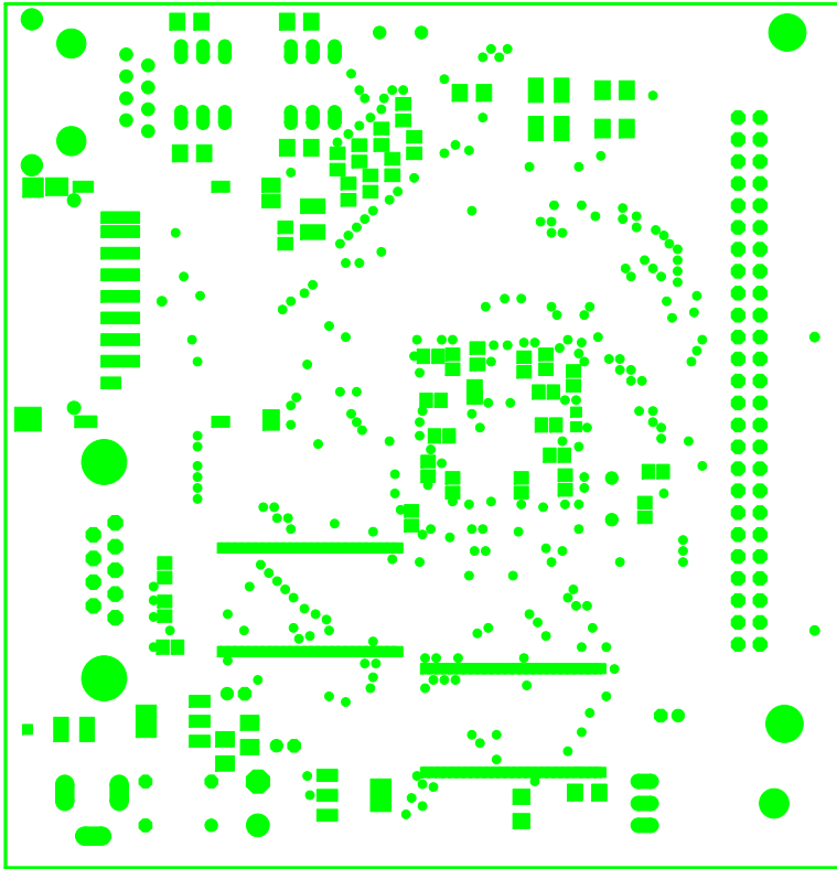
TOP SOLDERMASK
