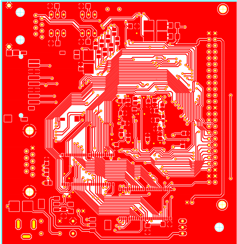
TOP COPPER
