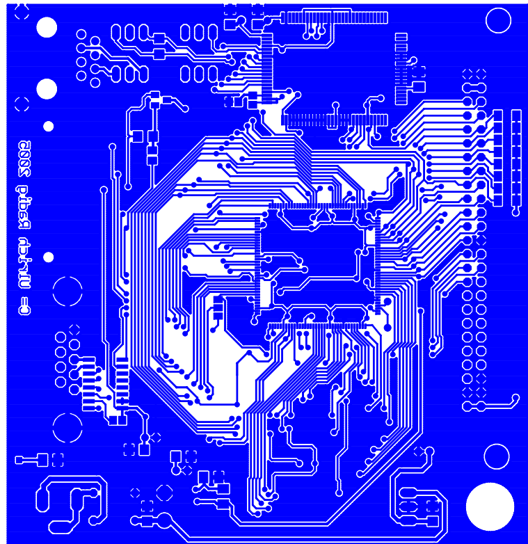
BOTTOM COPPER
